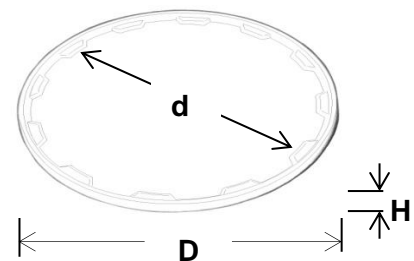
Standarddeckel
